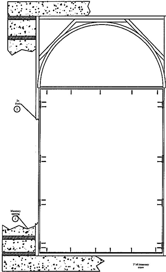
ANCHORING LAYOUT
